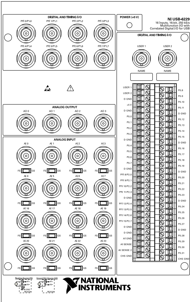
Figure 10. NI USB-6229 BNC Top Panel and Pinout
