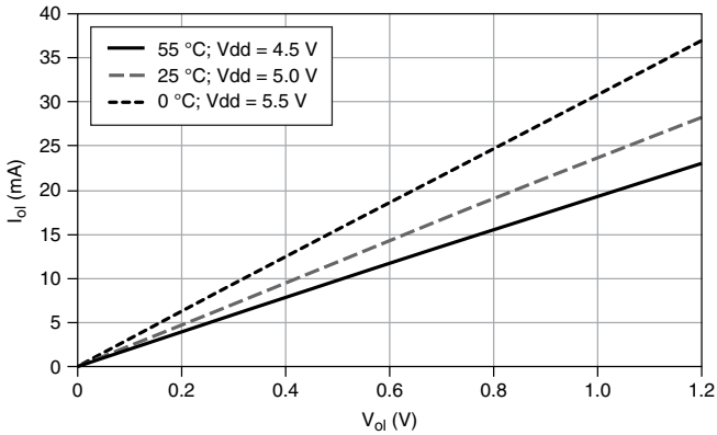
Figure 7. DIO PFI/Port 1/Port 2: I_{OI} versus V_{OI}
